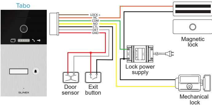
Diagram 3. Locks with external power supply connection.
