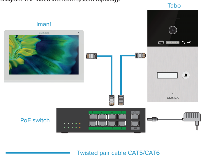
Diagram 1. IP video intercom system topology.
