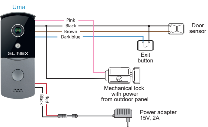
Diagram 2. Sensor, exit button, lock and power supply connection.
