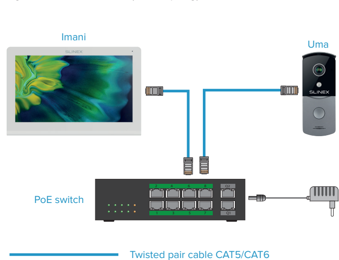
Diagram 1. IP video intercom system topology.
