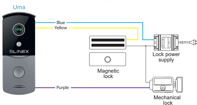
Diagram 3. Locks with external power supply connection.
